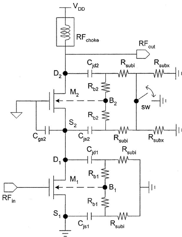
Fig. 2. Cascode amplifier with substrate parasitics.
